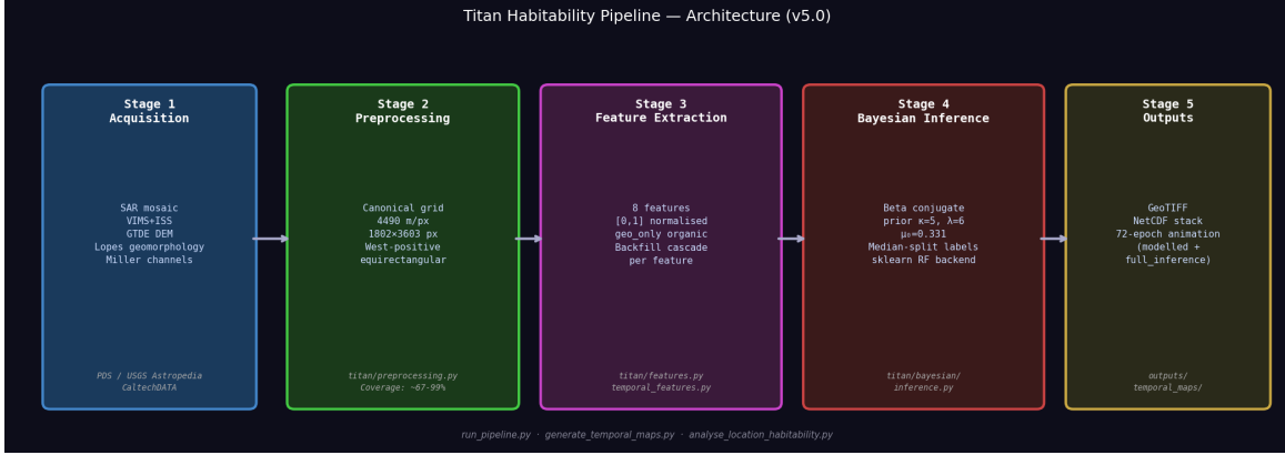
Figure E.1: Schematic overview of the five-stage Titan habitability analysis pipeline. All eight habitability-proxy features are extracted in Stage 3 and combined in the Bayesian posterior update of Stage 4 to produce P(H | \mathbf{f}) maps at each of the five temporal configurations.
