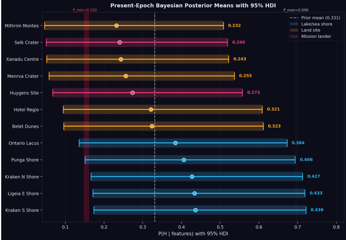
Figure 3.2: Present-epoch posterior means P(H | \mathbf{f}) with 95% highest-density intervals (HDI) for twelve representative Titan surface environments, computed from the Bayesian formula (Eq. 2.8). Cyan bars = lake/sea shore sites; amber bars = land sites. The dashed vertical line marks the prior mean \mu_0 = 0.331 . The shaded red band marks the prior floor P_{\min} = 0.150 . Note that the HDI widths are similar for all sites ( \sim 0.4 – 0.6 units wide), reflecting the weak concentration \kappa = 5 ; only the location of the interval changes with the feature data. Polar lake shores are unambiguously separated from equatorial land sites by \sim 0.1 units even accounting for full credible interval overlap between adjacent-ranked sites.
